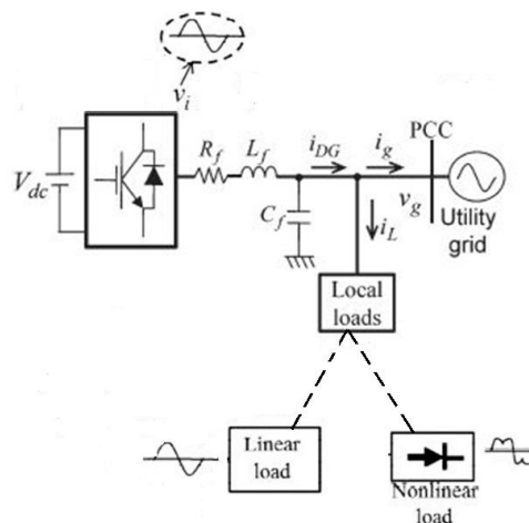
Fig. 1. Connection interface of DG with various loads
