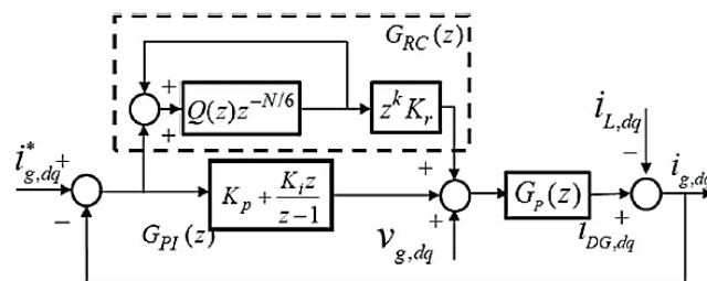
Fig. 4. Block diagram of PI-RC current controller
