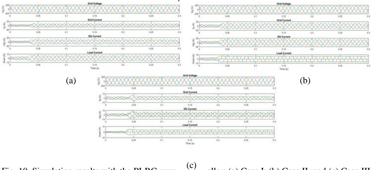
Fig. 10. Simulation results with the PI-RC current controller: (a) Case I; (b) Case II; and (c) Case III.
