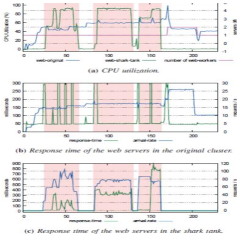
Figure 4: DDoS mitigation. Attack periods are shown in shaded background. FVDAMP redirects the suspicious traffic to the shark tank on the fly.
